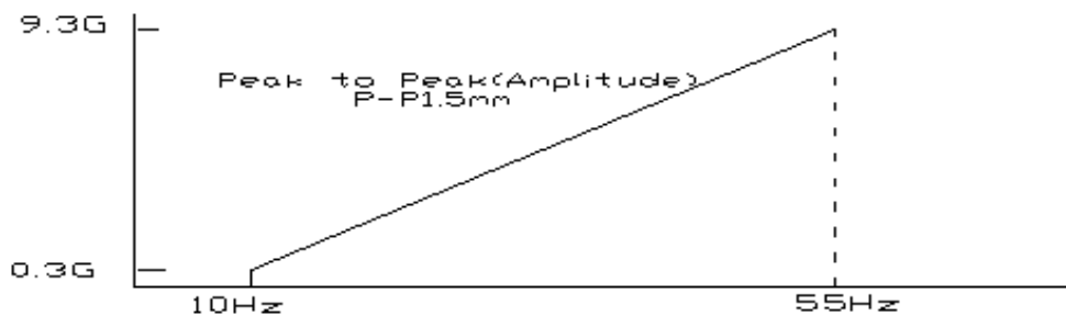
FIG 5 VIBRATION TEST
